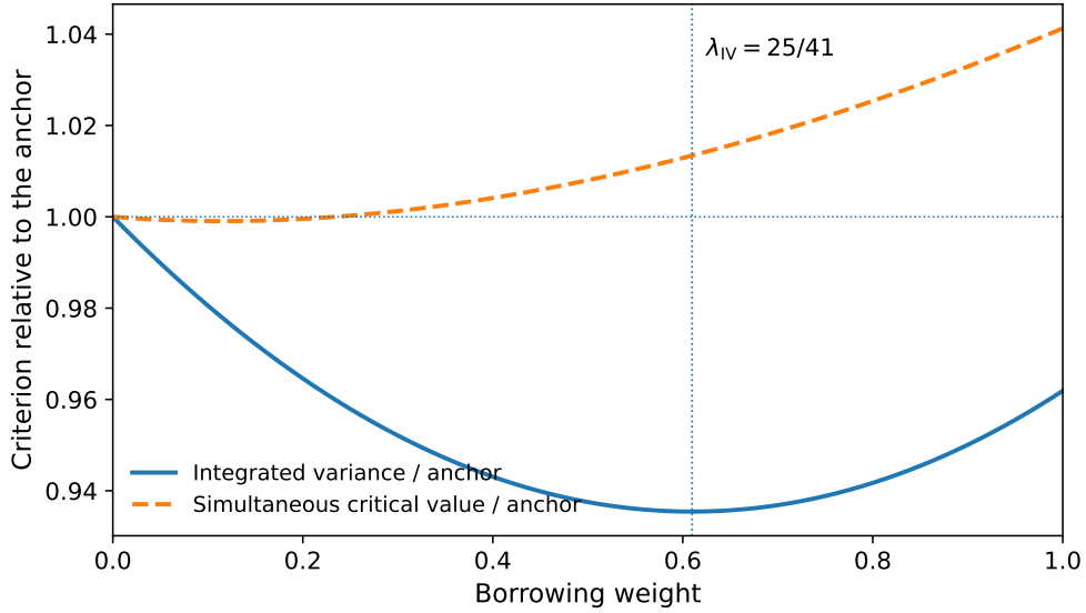
Figure 1: The exact two-threshold example separates the trace and simultaneous-band criteria. Both curves are relative to Anchor; at the trace optimum 25/41 , the simultaneous critical value exceeds the anchor value. These are Gaussian calculations, not Monte Carlo estimates.
