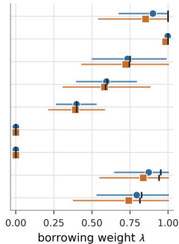
(c) Borrowing-weight recovery
