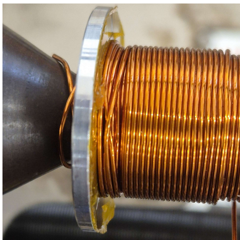
(a) Coil end error 1
