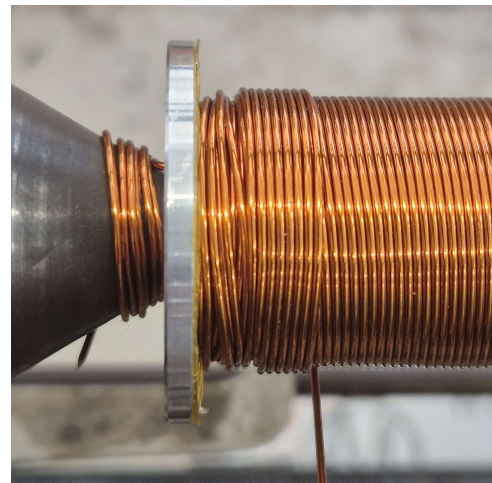
(b) Coil end error 2
