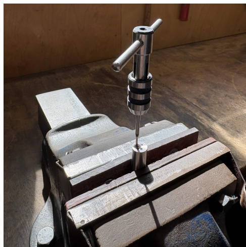
(a) Tapping of central iron core baseplate-connecting holes
