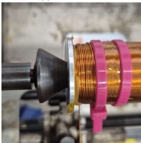
(c) Coil end error 3 and fix solution
