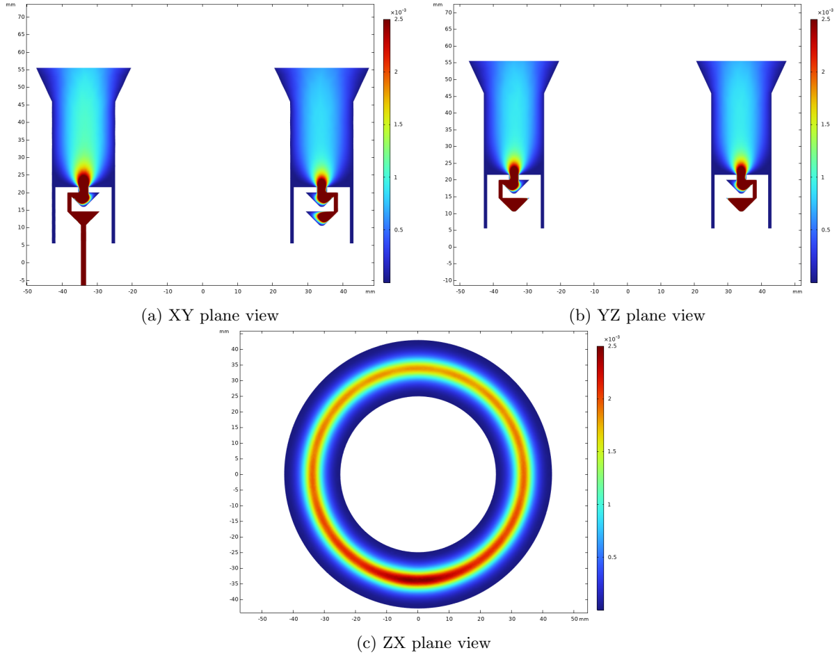
Figure 8: Orthogonal COMSOL cross-sections of the anode geometry showing gas distribution pathways.
