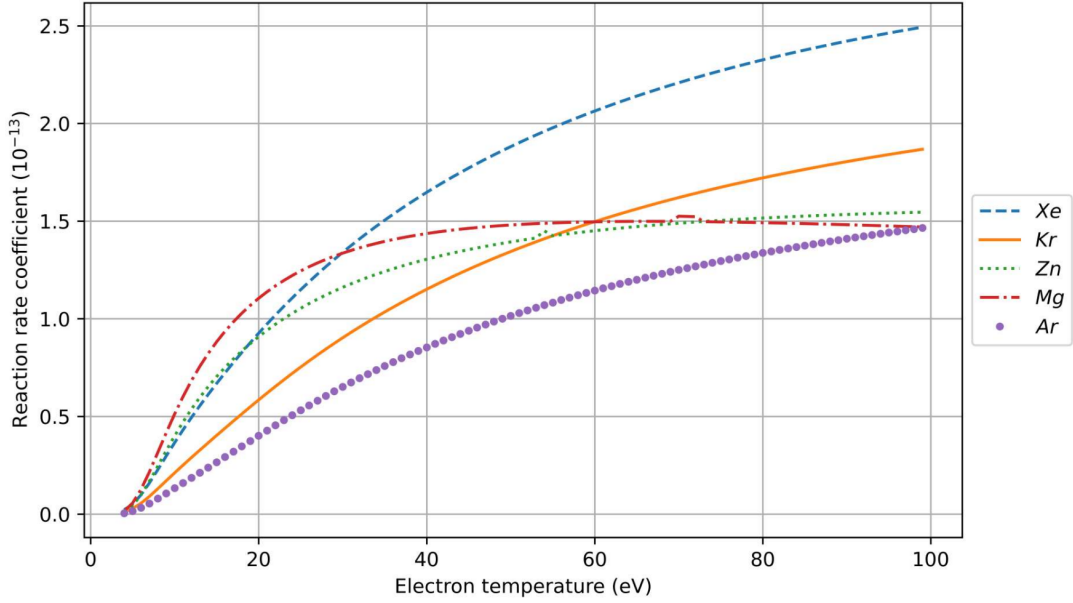
Figure 2: The calculated reaction rate coefficient against bulk electron temperature for propellants: Xenon, Krypton, Zinc, Magnesium and Argon (2)
