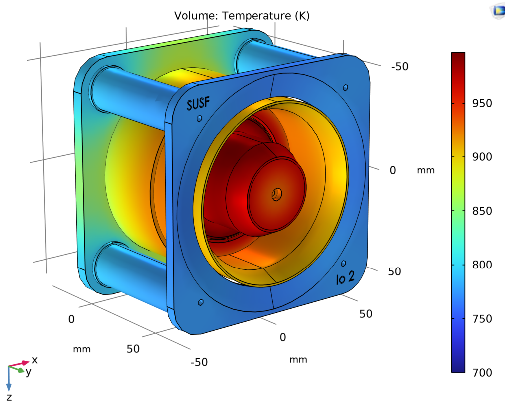
Figure 9: Temperature distribution for Io2.
