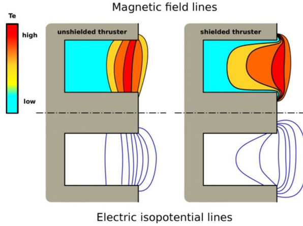
Figure 3: Illustration of the magnetic field isolines along with the electron temperature distribution in the channel for unshielded topologies (left) and shielded (right)(4) .
