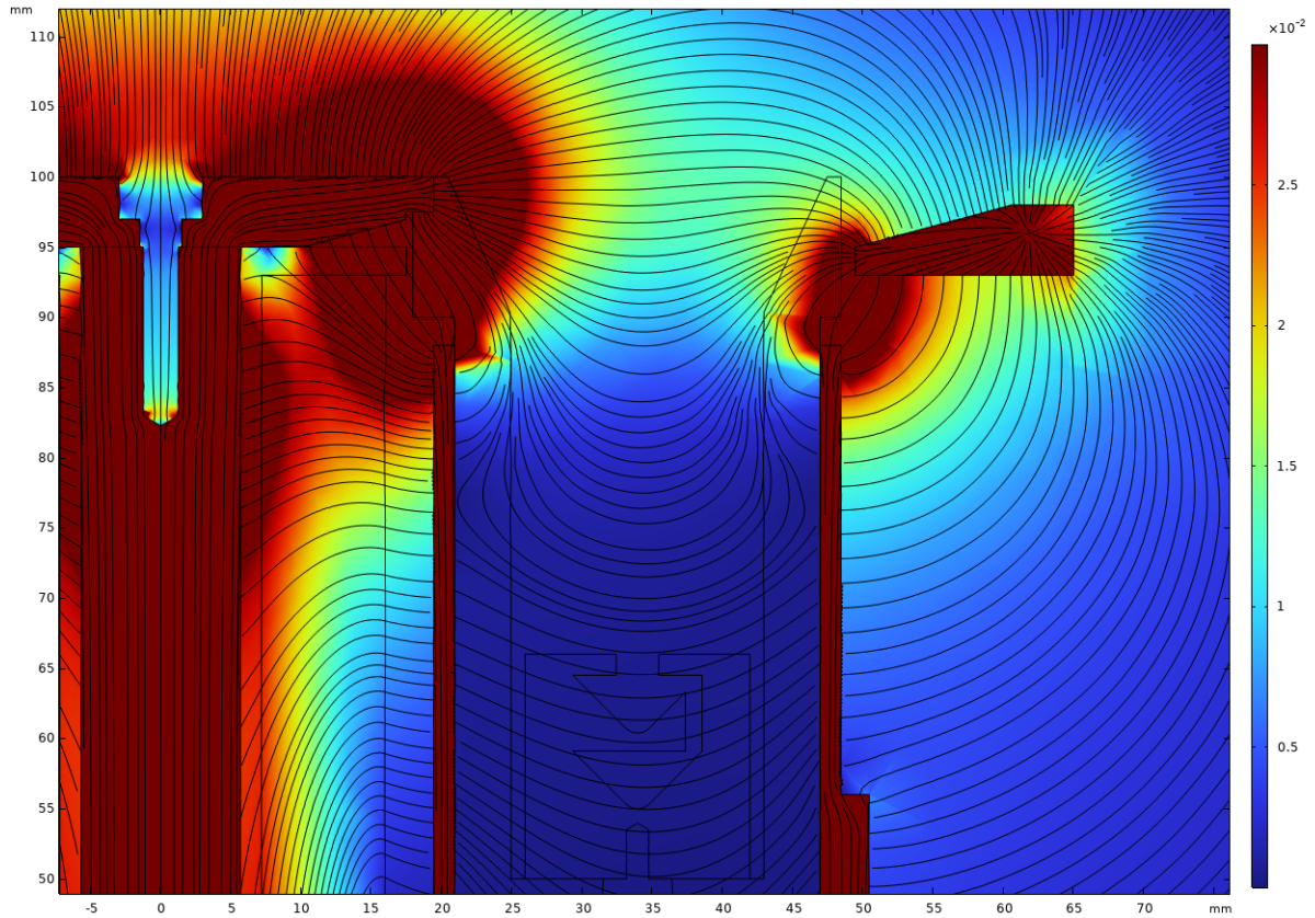
Figure 5: Magnetic Field Contour
