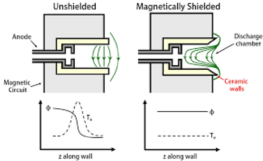
Figure 4: Illustration of the magnetic field isolines along with the electron temperature and potential distribution along the axial wall of the discharge channel for unshielded topologies (left) and shielded (right) (5).
