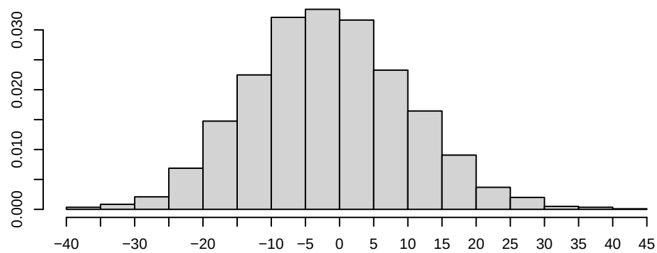
Density of mutual
