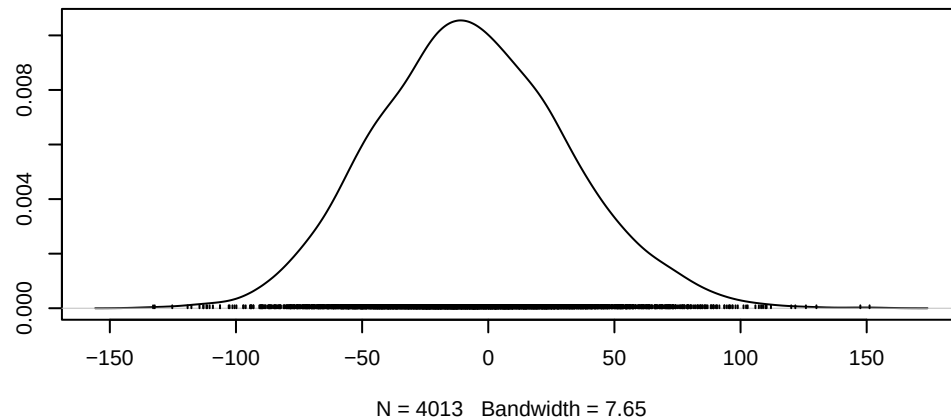
Density of gwesp.OTP.fixed.0.2
