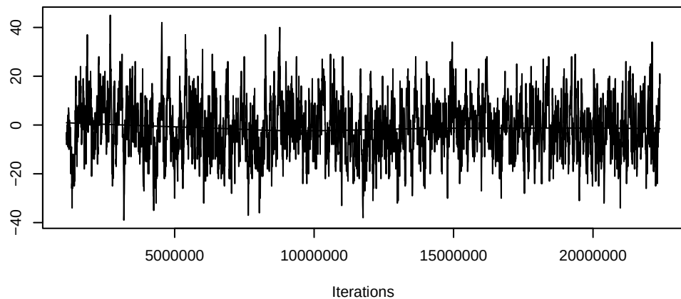
Trace of mutual
