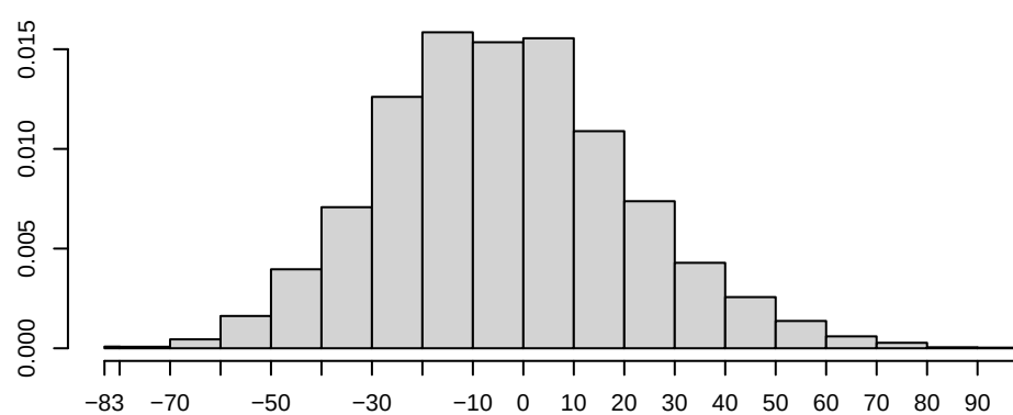
Density of nodeifactor.gender.1
