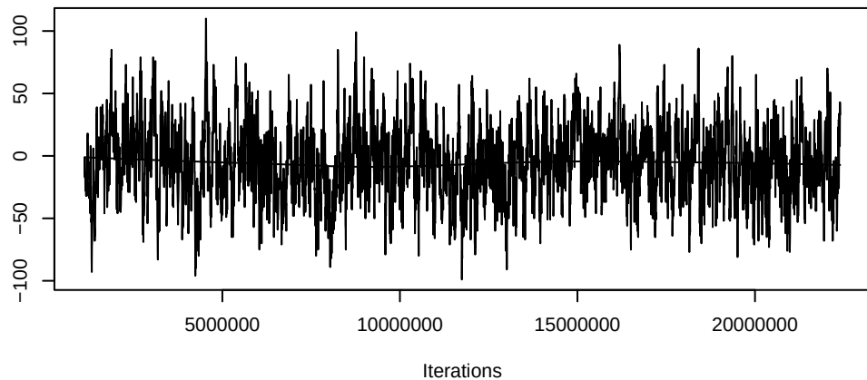
Trace of nodematch.gender
