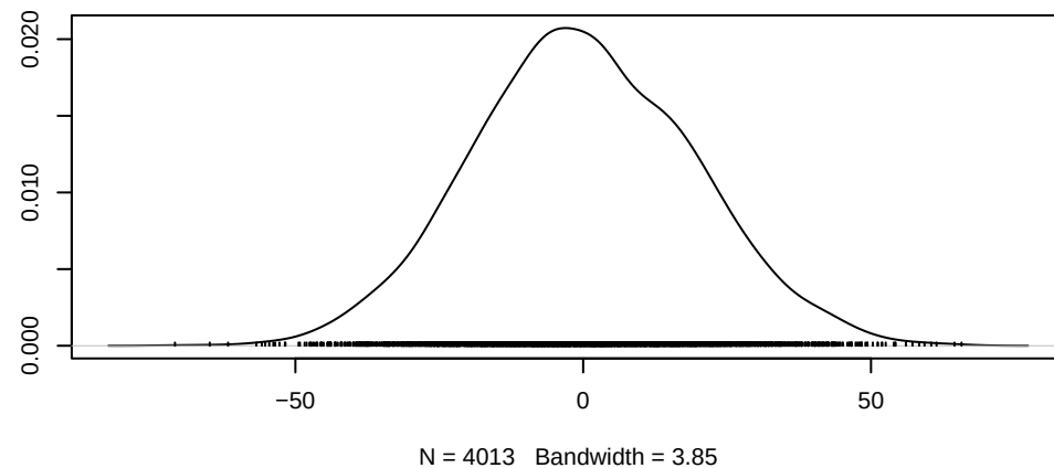
Density of edgecov.logdistance
