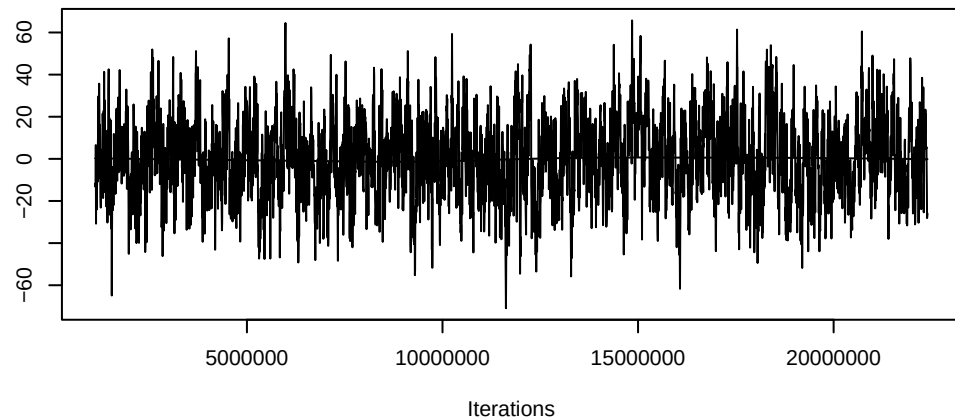
Trace of edgecov.logdistance
