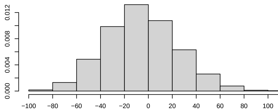
Density of nodematch.gender
