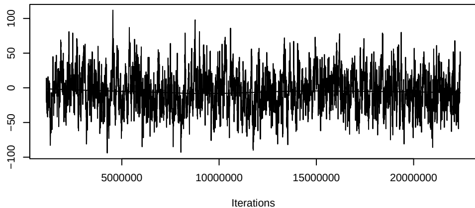
Trace of edges
