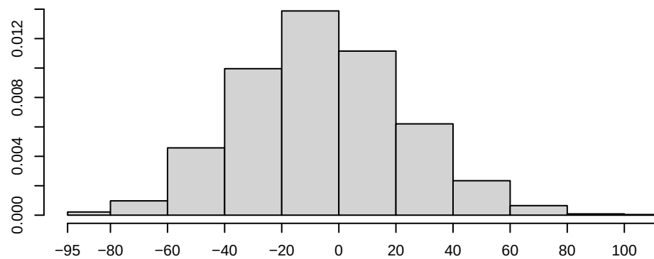
Density of edges
