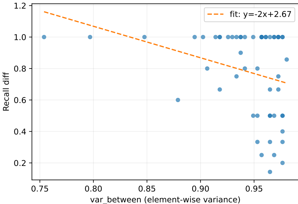
blend vs full reuse — Recall
