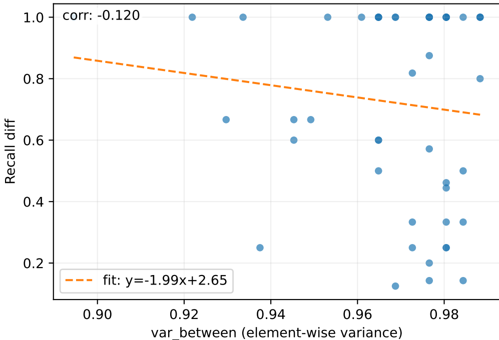
blend vs full prefill — Recall
