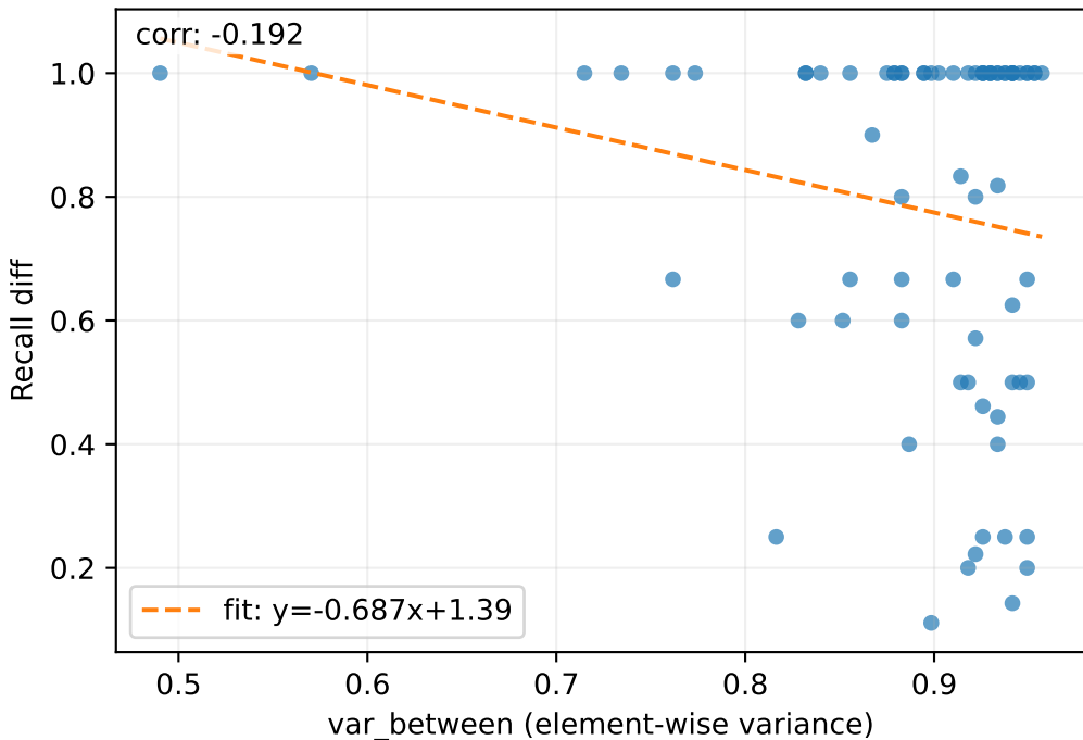
full reuse vs full prefill — Recall
