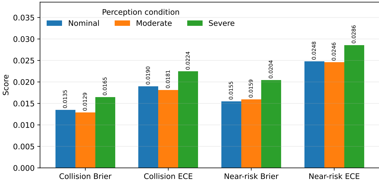
Aggregate probability quality of SAC-UPO-TTC
