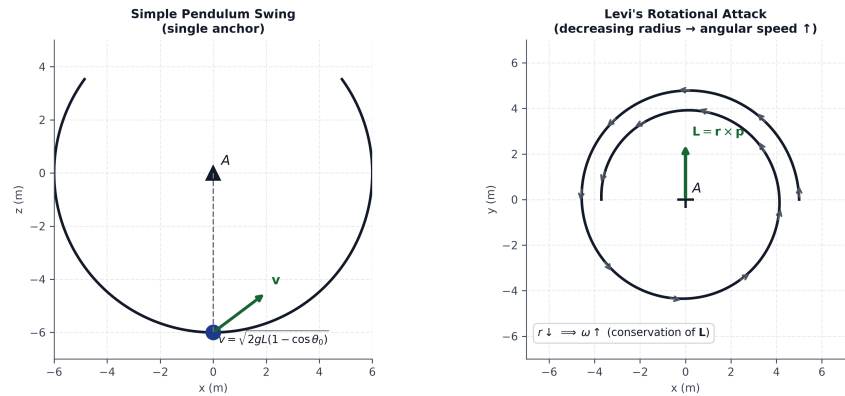
Figure 10b: Angular momentum conservation during radial cable retraction. Spiral path accelerates angular velocity. [MODEL]
