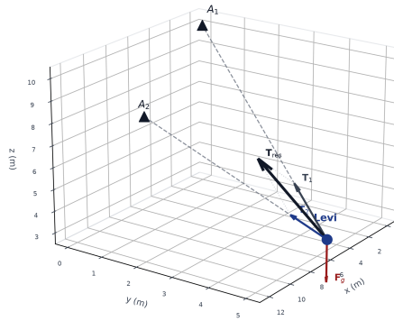
Figure 7b: Vector addition of dual cable tensions T_1 and T_2 producing controllable resultant T_{res} . [MODEL]
