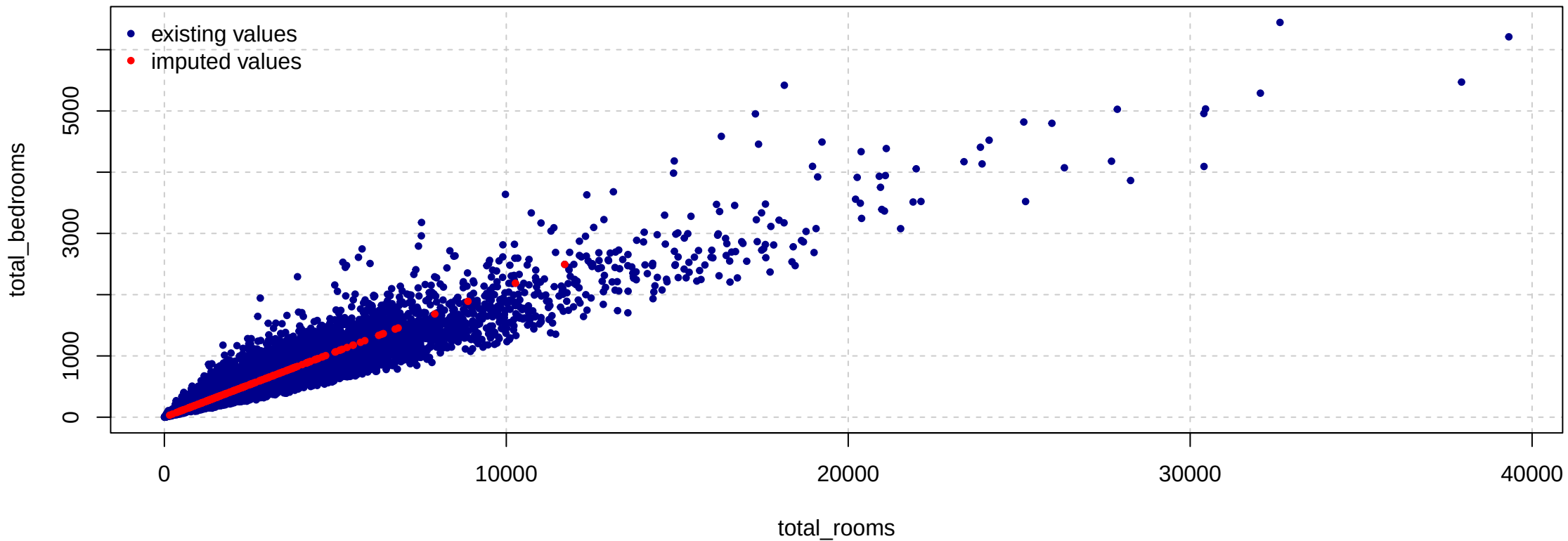
Comparison of total_rooms and total_bedrooms with imputed values
