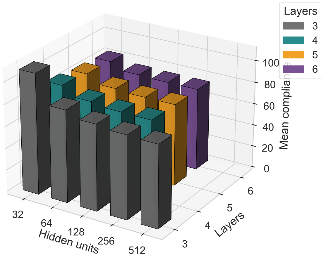
Mean compliance by architecture
