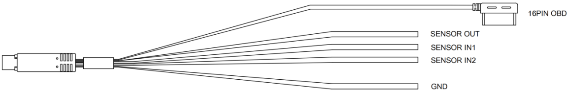
16PIN OBD Power Cable — Optional
