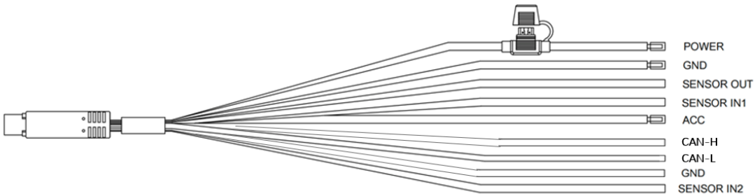
ACC Power Cable
