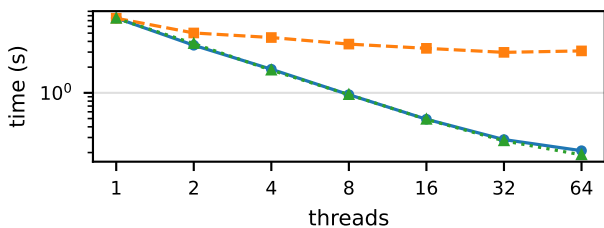
mode 5 (dimension=365)
