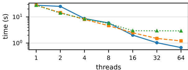
mode 6 (dimension=10)
