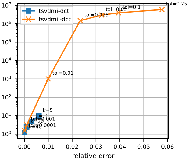
NCEP Air 6-way
