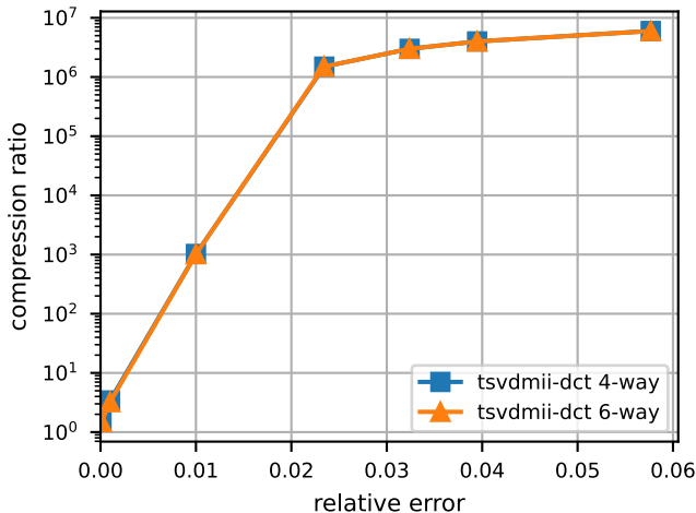
ncep-air: compression ratio (4-way vs 6-way)
