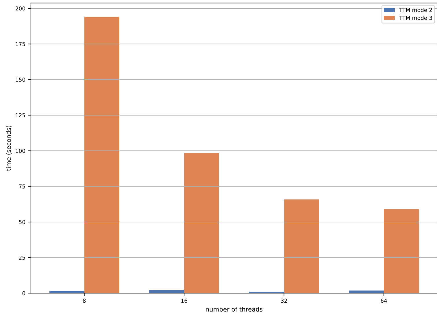
NCEP Air — Compress TTM Strong Scaling (tsvdmii-dct, tol=0.01)
