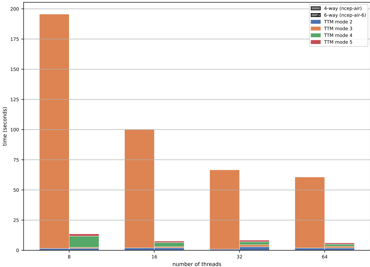
NCEP Air — Compress TTM Strong Scaling: 4-way vs 6-way (tsvdmii-dct, tol=0.01)
