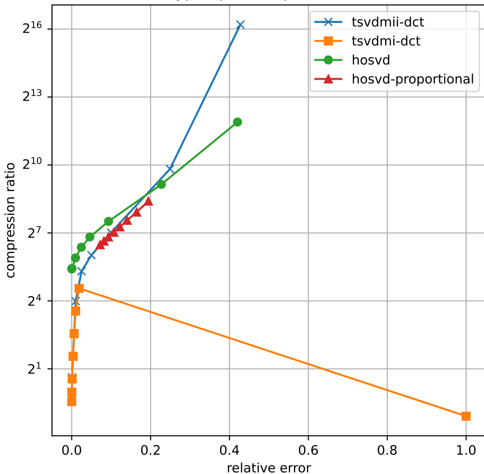
DC Mall Hyperspectral, perm-mode=(0,2,1)
