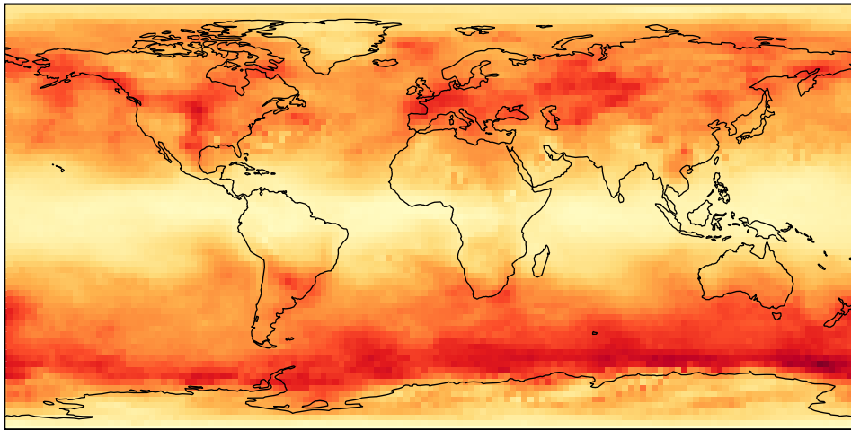
EOF — median relative error at extremes
