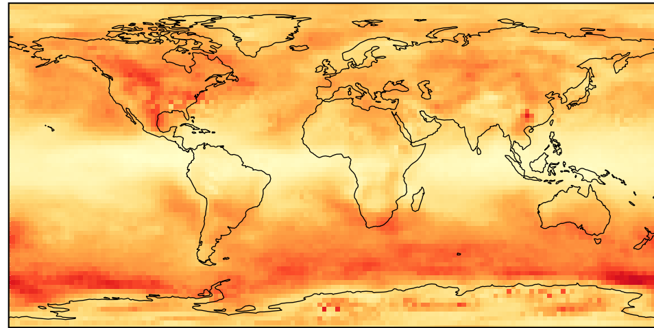
tsvdmii — median relative error at extremes
