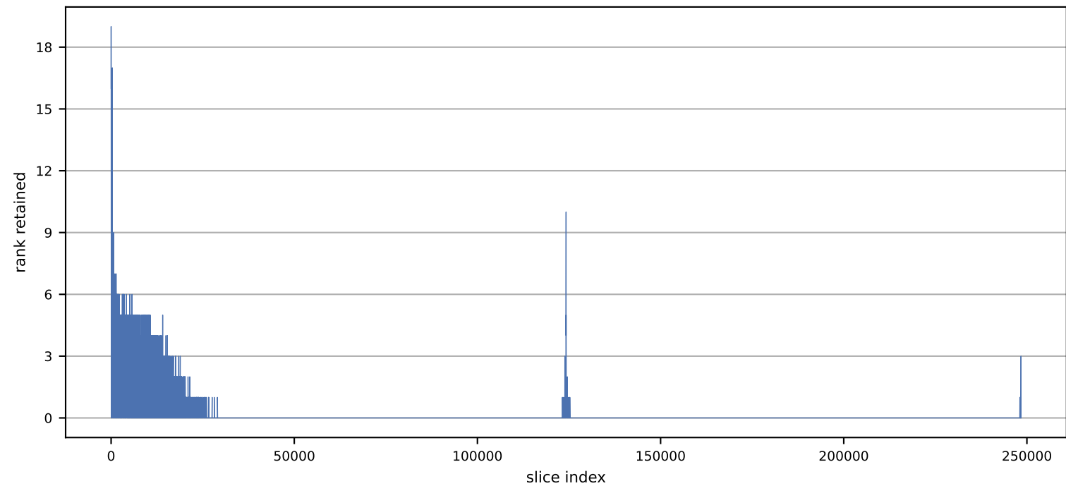
NCEP Air — Per-slice Rank Retained by tsvdmm (perm_mode=0123, 64 threads)
