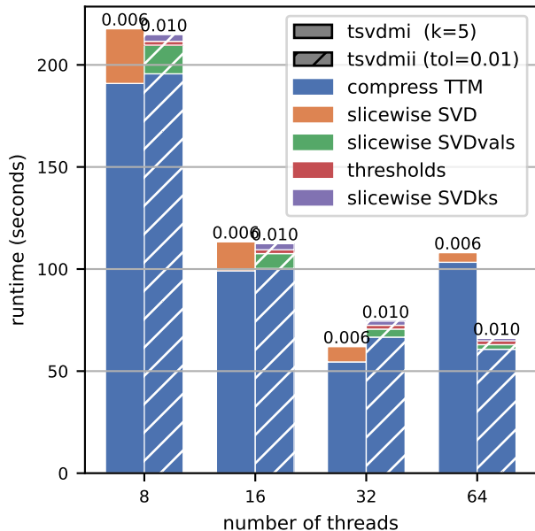
NCEP Air — Strong Scaling
