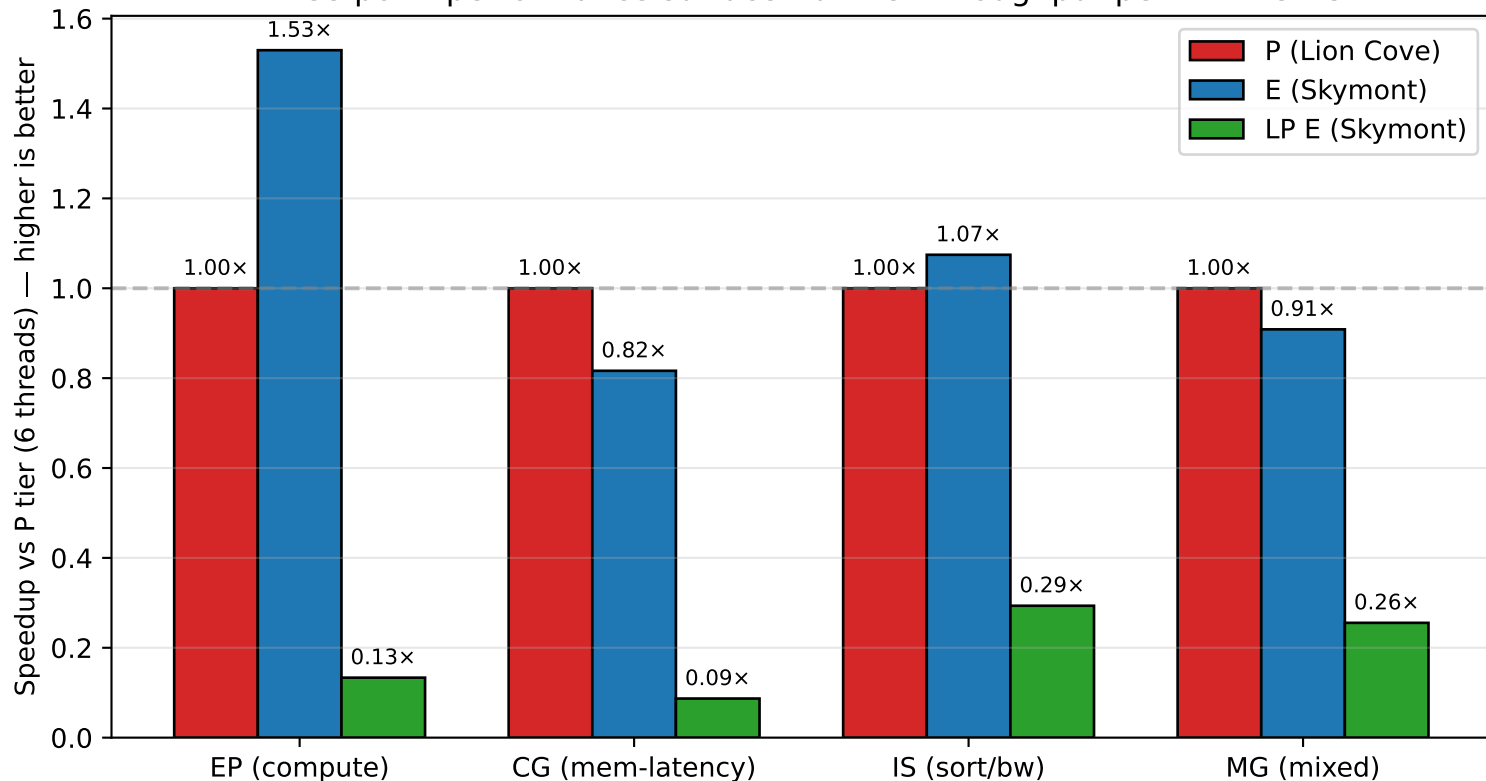
Three-point performance surface: full-tier throughput per NPB kernel
