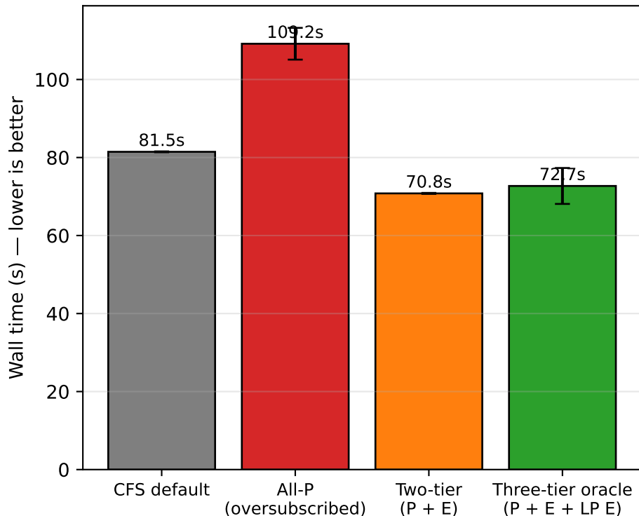
Time to complete mixed workload (6×cg.B + 4×ep.B + 2×stress-ng I/O)
