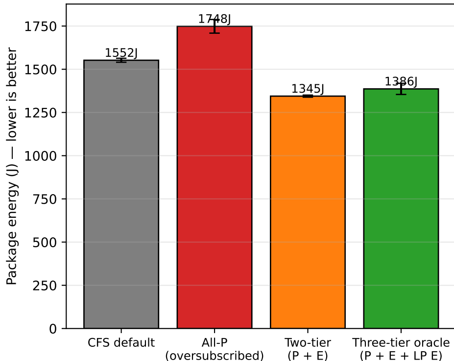
Total energy over the run (Intel RAPL package domain)
