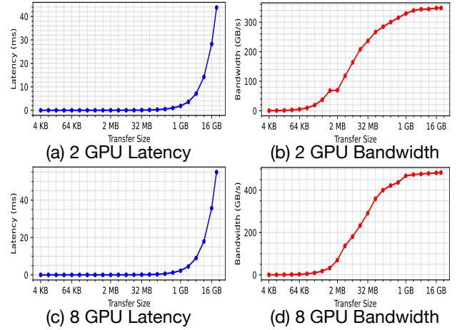
Fig. 7. Average latency (a, c) and bandwidth (b, d) for NCCL Allreduce with 2 and 8 receiver GPUs in NVLink 4.0
