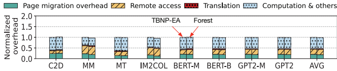
Fig. 5. Performance breakdown normalized to TBNP-EA
