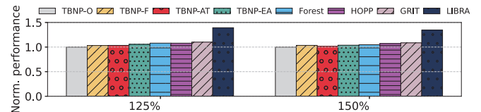
Fig. 24. Memory oversubscription performance
