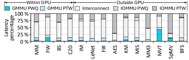
Fig. 5: Latency breakdown of page table walk requests.
