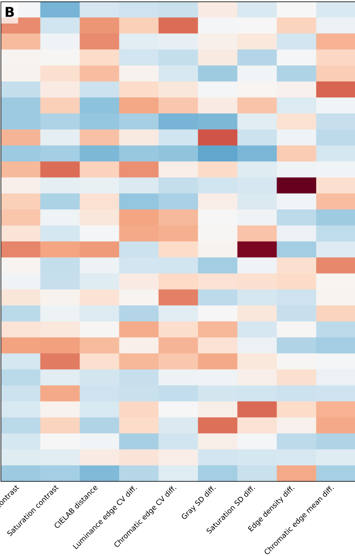
Animal-background detectability
