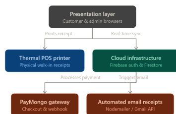
Fig. 4.22 Serverless Client-Cloud Architecture Diagram for Mrs. Brave's Cakes
