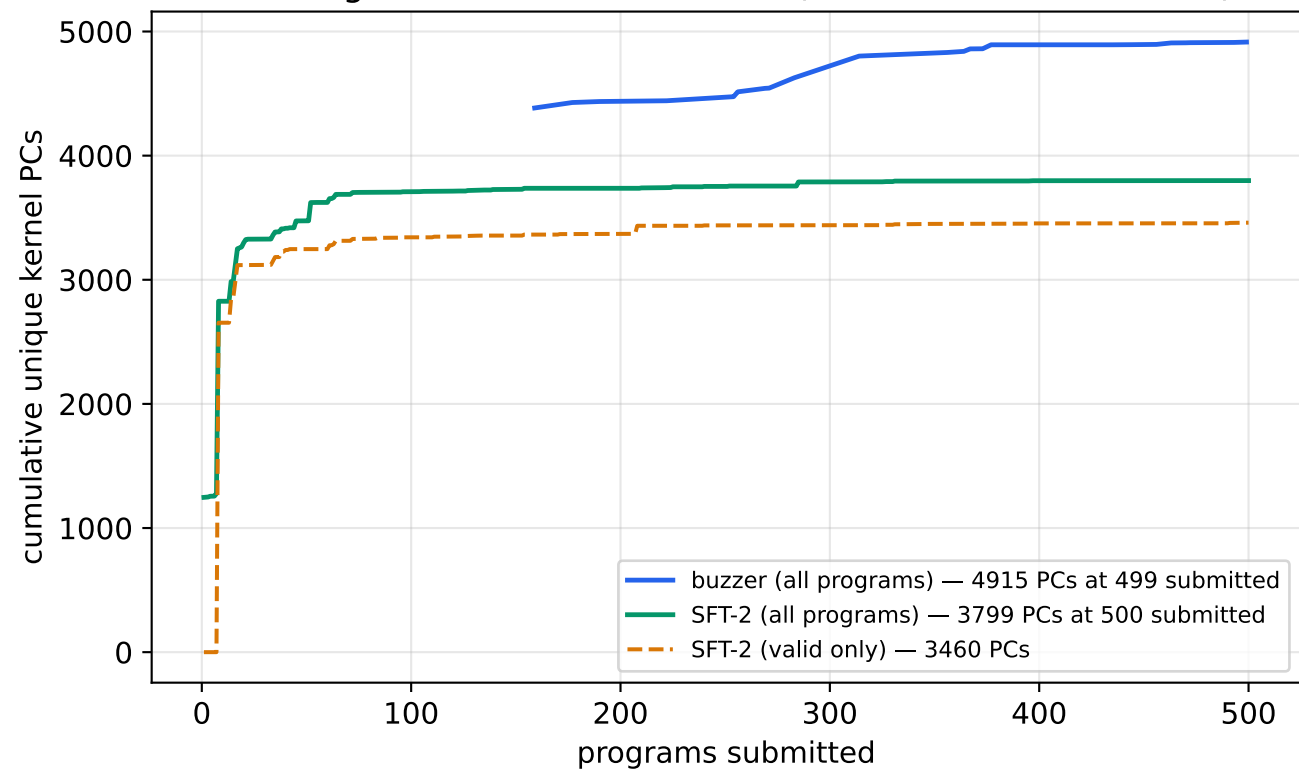
Coverage race: buzzer vs. SFT-2 (confounded — see text)
