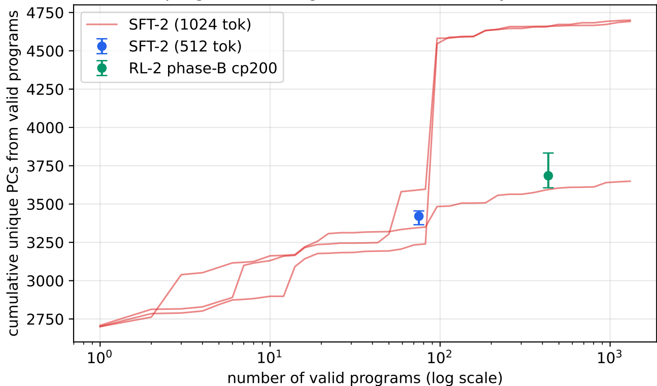
Valid-program coverage saturates (diversity is the wall)
