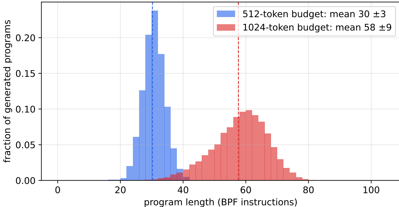
SFT-2 program length: narrow, and pinned by the token budget
