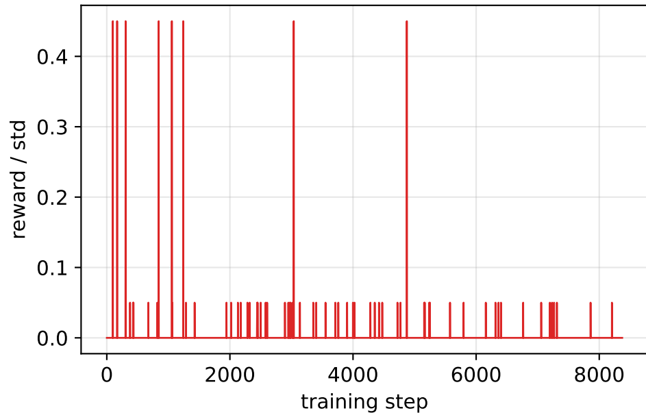
RL-1 (grpo-rl-v1, 8,373 steps)
