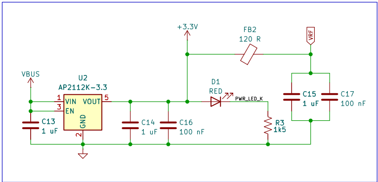
3V3 POWER REGULATOR
