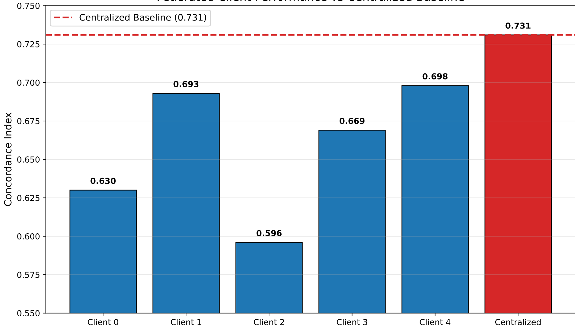
Federated Client Performance vs Centralized Baseline
