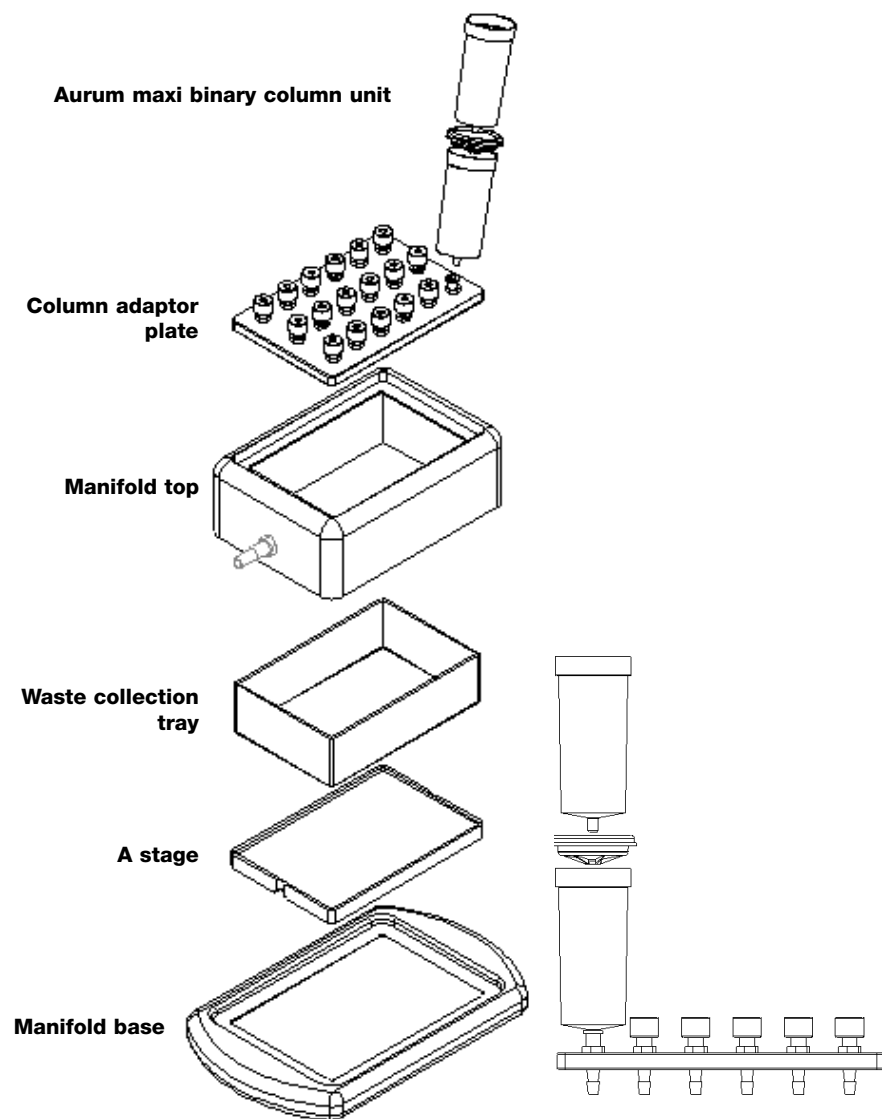
Fig. 3a. Vacuum setup conditions for the Aurum plasmid maxi kit
