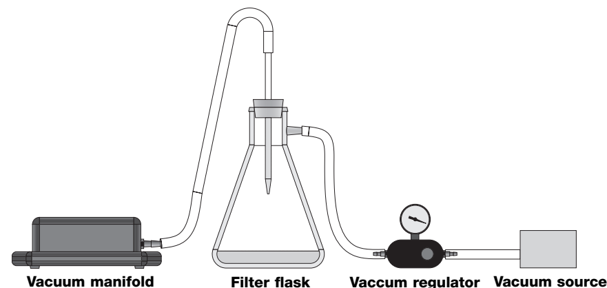
Fig. 4. Vacuum setup conditions
