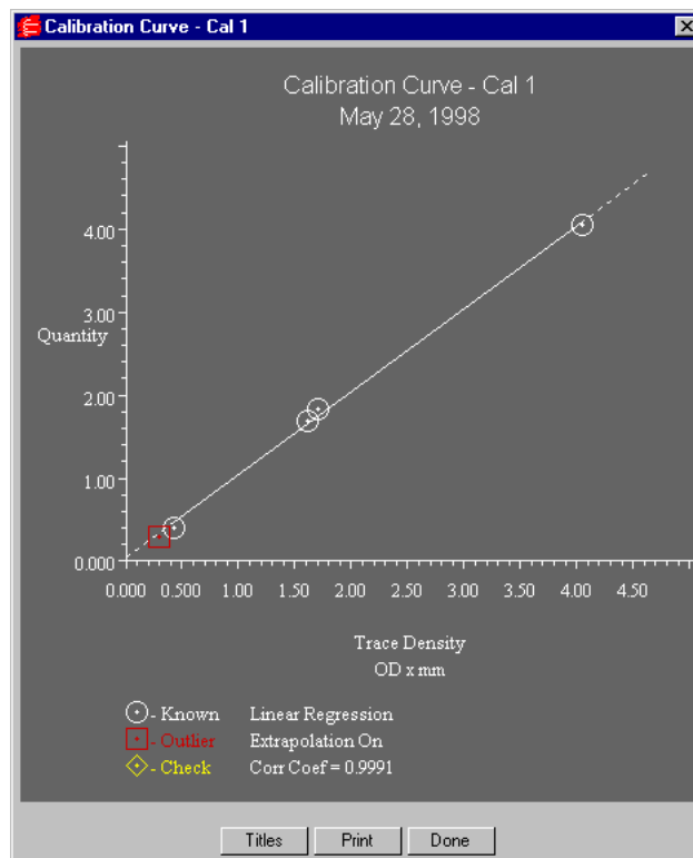
Fig.14-21. Calibration curve with titles displayed, linear regression, and extrapolation.
