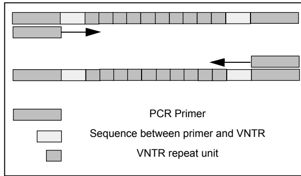
Fig.17-4. Diagram of components of a DNA fragment.
