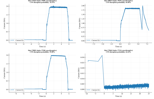
(b) Four selected non-disruptive shots incorrectly identified as disruptive by the CNN. Shots 178891 and 176423 have a drop that somewhat resembles a disruption, confusing the model. Notice that the CNN disruption probability is lower for the more confusing shots.
