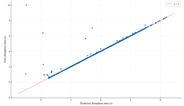
Figure 4: Predicted disruption time Eq (7) vs real disruption time for 889 test holdout shots. We see a few outliers, with the majority of predictions on the accurate y = x line.
