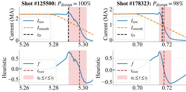
Figure 6: Two example shots (above) with their disruption heuristic f(t) (below). On the left, we see shot #125500 with a DIII-D label near the disruption start (Eq (??)); on the right, we see shot #178323 with a DIII-D label near the disruption root (Eq (??)).
