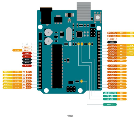
5 Connector Pinouts
