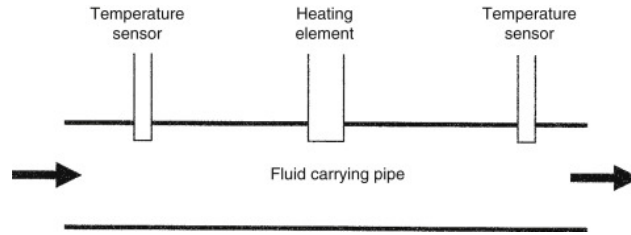
Figure 2: Structure of thermal mass flowmeter.
