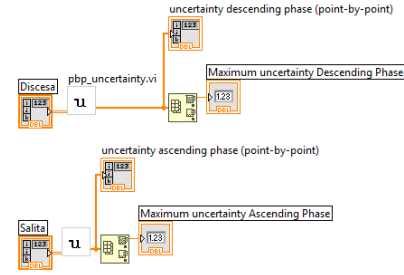
(b) uncertainty_datasets.vi SubVI Block Diagram
