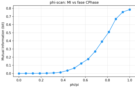
FIG. 3. Mutual information as a function of controlled-phase angle \phi for the standard PASM protocol on ibm_marrakesh. The modulation confirms the phase origin of the correlation.
