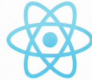
React
