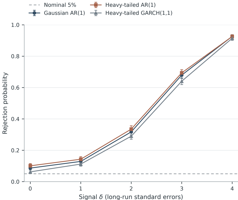
(b) Max-test power: one strategy has a positive mean
