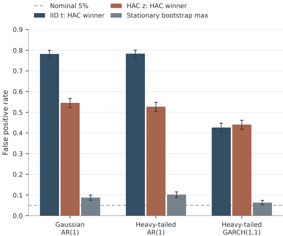
(a) All strategy means are zero
