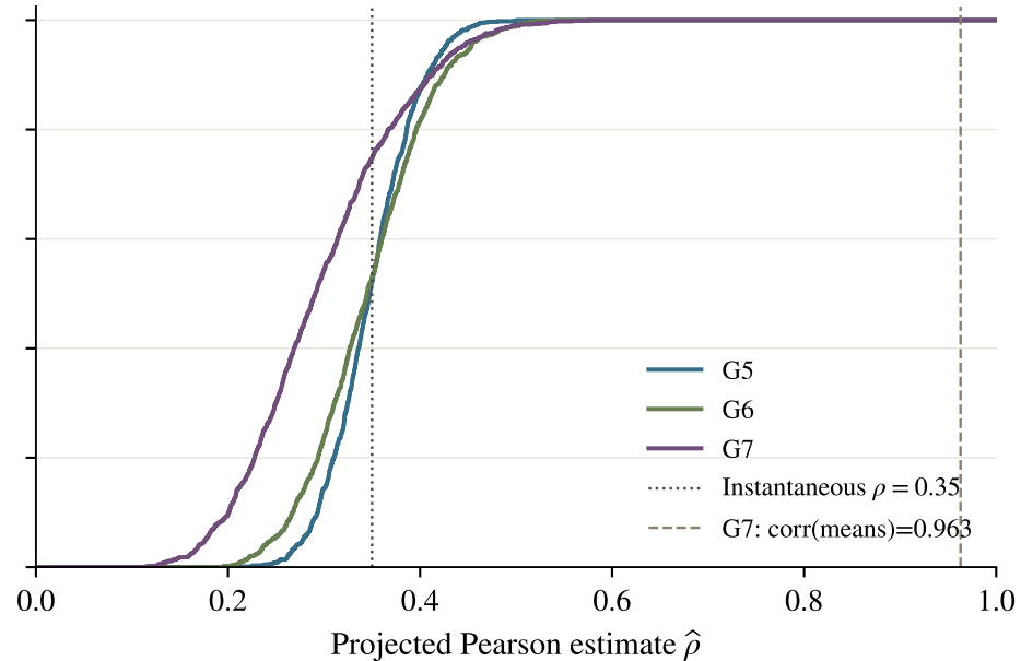
(b) Cross-candidate correlation
