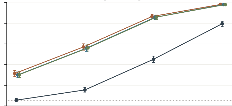
(b) G7: Temporal misspecification
