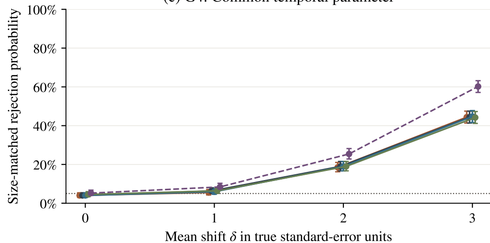
(c) G4: Common temporal parameter
