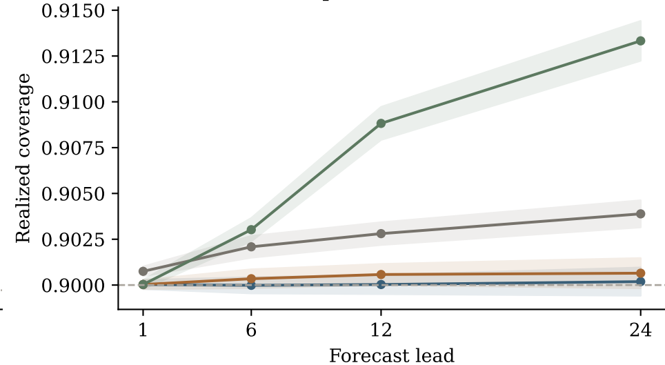
Abrupt variance shifts
