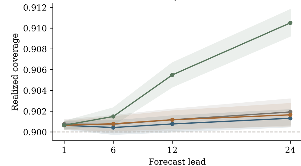
Fast volatility (stress test)
