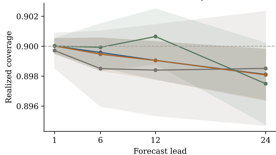
Abrupt variance shifts
