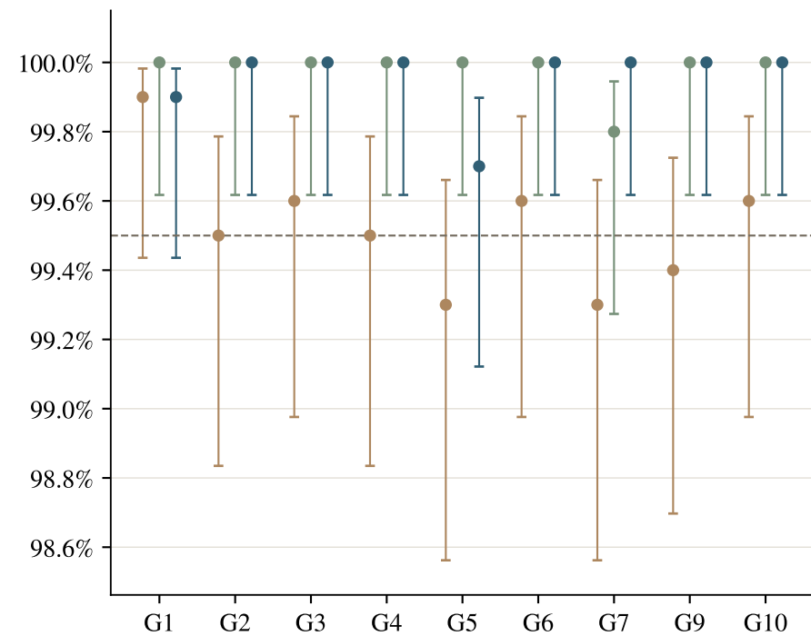
Common-coefficient coverage (zoomed axis)
