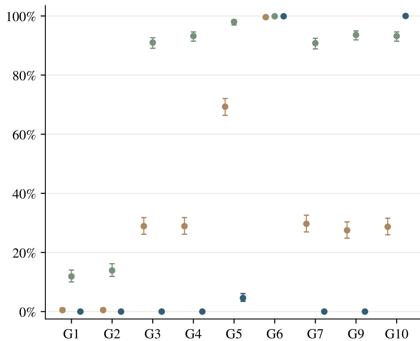
Outer set retains \phi = 1
