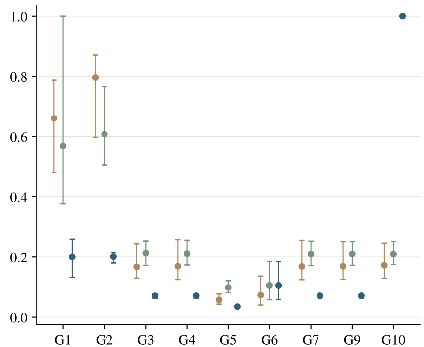
CI width: median and 10–90% range
