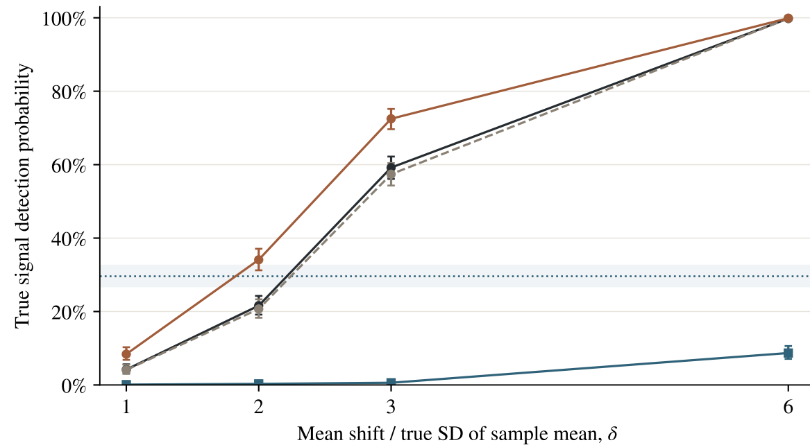
G5: T = 1024 , \phi = .96875 , K = 20
