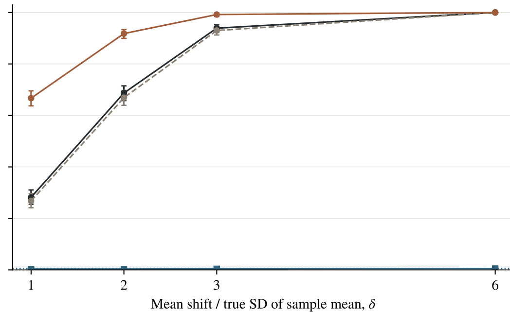
G6: T = 200 , \phi = .99 , K = 1
