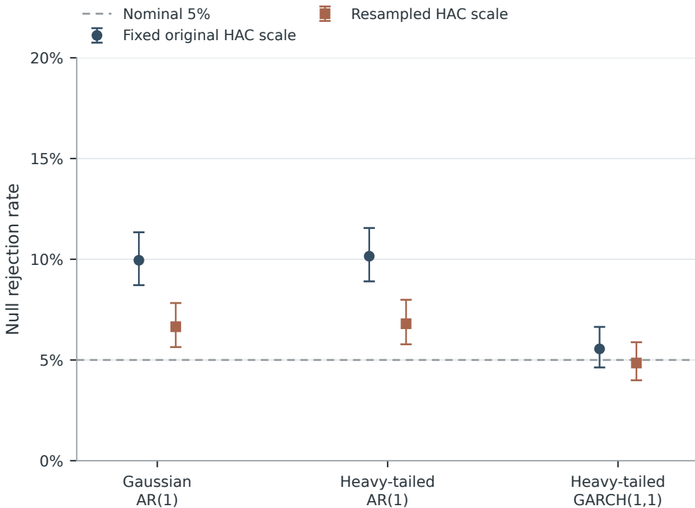
(a) All strategy means are zero
