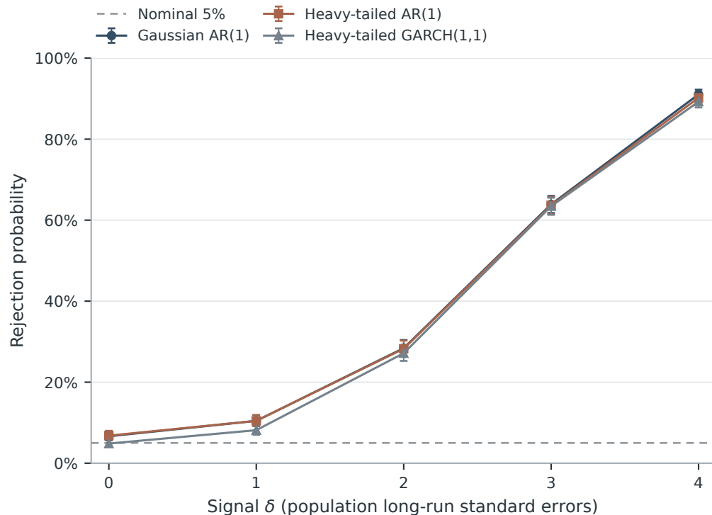
(b) Resampled-HAC max test: one positive mean
