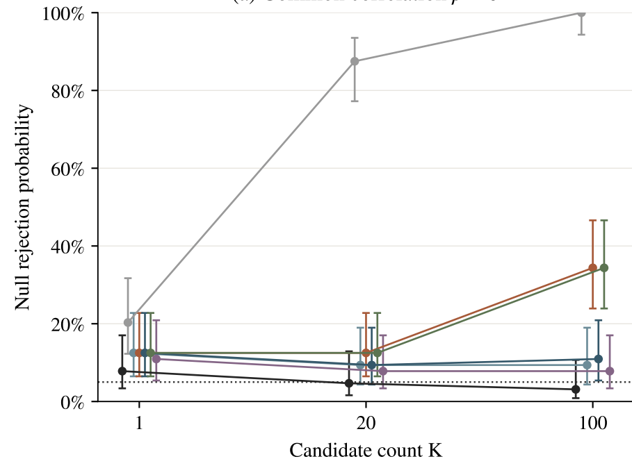
(a) Common correlation \rho = 0
